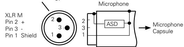
Connection diagram of measurement microphones with electronic data sheet
