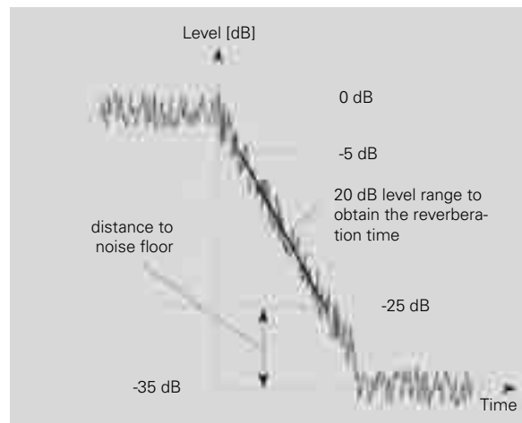
RT60 Measurement with T20 method
