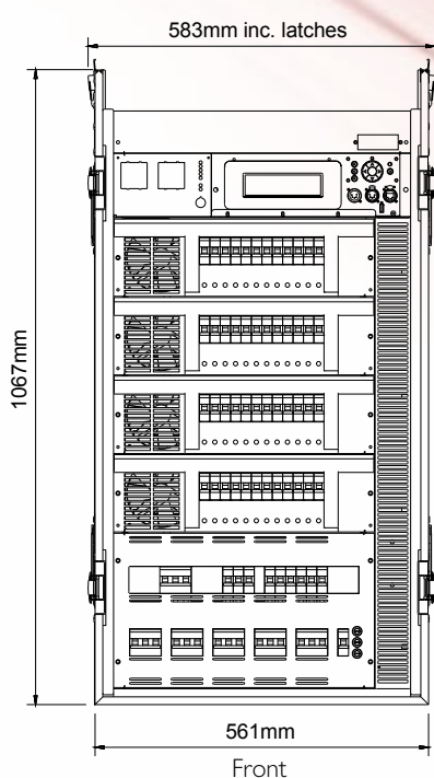
ART2000 T4 dimensions - other versions may vary
