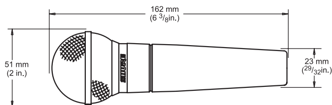
OVERALL DIMENSIONS
