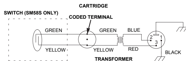
INTERNAL CONNECTIONS
