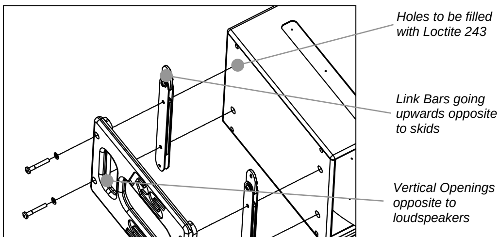
INSTALLING RS15 FLYING PLATES AND HANDLES
