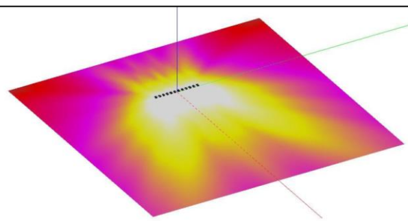
STRAIGHT DELAYED SUBWOOFER ARRAY ACROSS STAGE
