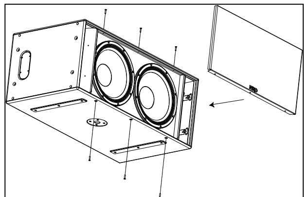
CONFIGURING RS15 AS LEFT
