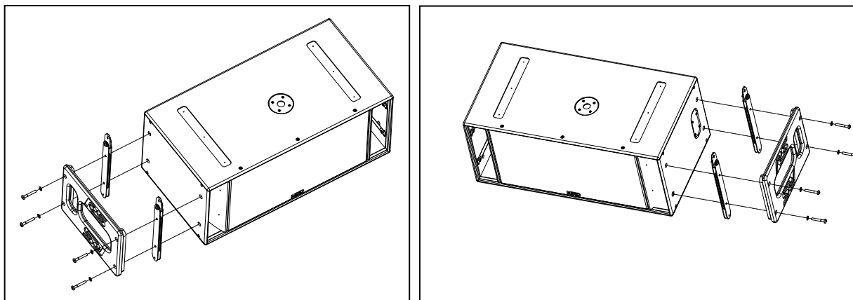
INSTALLING RS15 FLYING PLATES AND HANDLES
