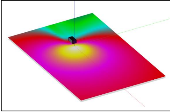
HORIZONTAL COVERAGE IN DIRECTIONAL MODE (100 HZ)
