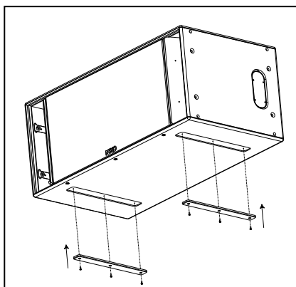
CONFIGURING RS15 AS RIGHT
