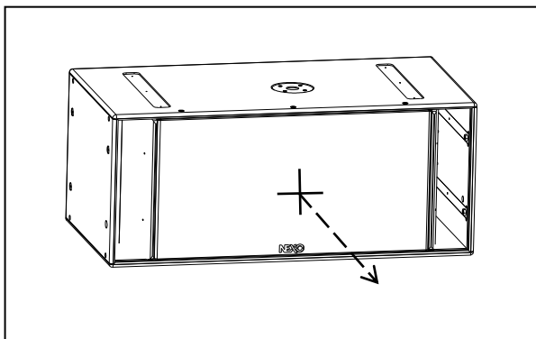
RS15 REFERENCE POINT IN OMNI MODE
