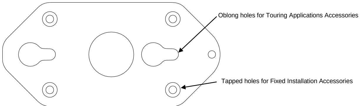
PS10R2 AND PS15R2 CONNECTING PLATES
