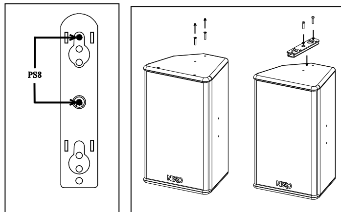
PS8 FLYING ADAPTOR INSTALLATION
