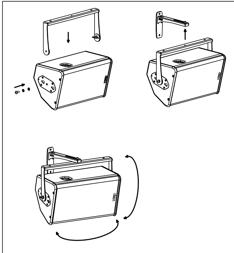
WALL SUSPENSION PROCEDURE FOR HORIZONTAL INSTALLATION
