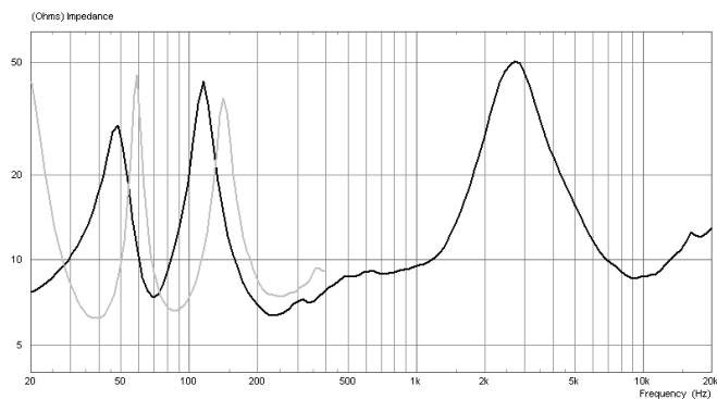
Impedance LS600 (grey) & PS10 (black)
