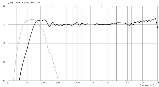
On-axis response RS15 (grey) & PS15 (black)
