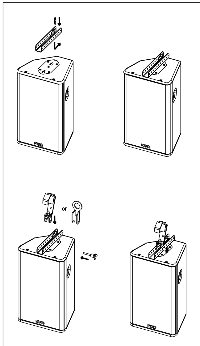
PS SERIES VERTICAL SUSPENSION PROCEDURE
