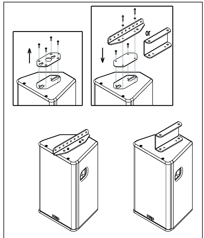
CABLE SUSPENSION MOUNTING PROCEDURE 2
