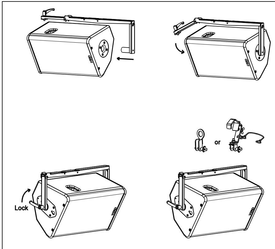
PS SERIES HORIZONTAL SUSPENSION PROCEDURE
