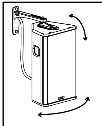
WALL SUSPENSION PROCEDURE FOR VERTICAL INSTALLATION
