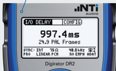
Channel propagation delay measurement
