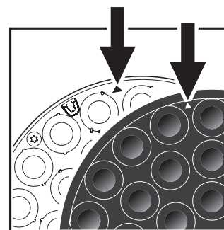
Figure 6: Alignment arrowheads
