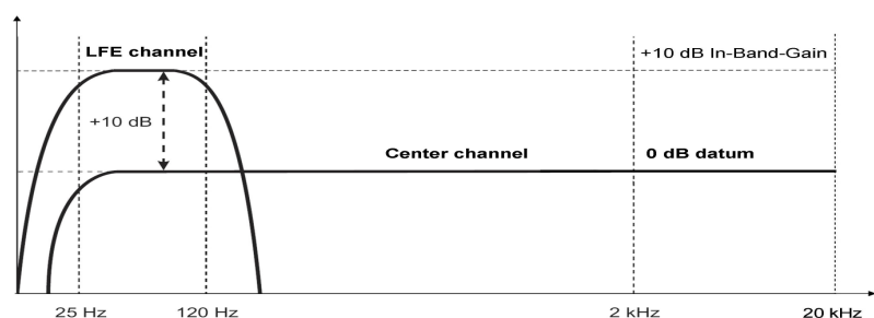
Level alignment of LFE and surround sound speakers
