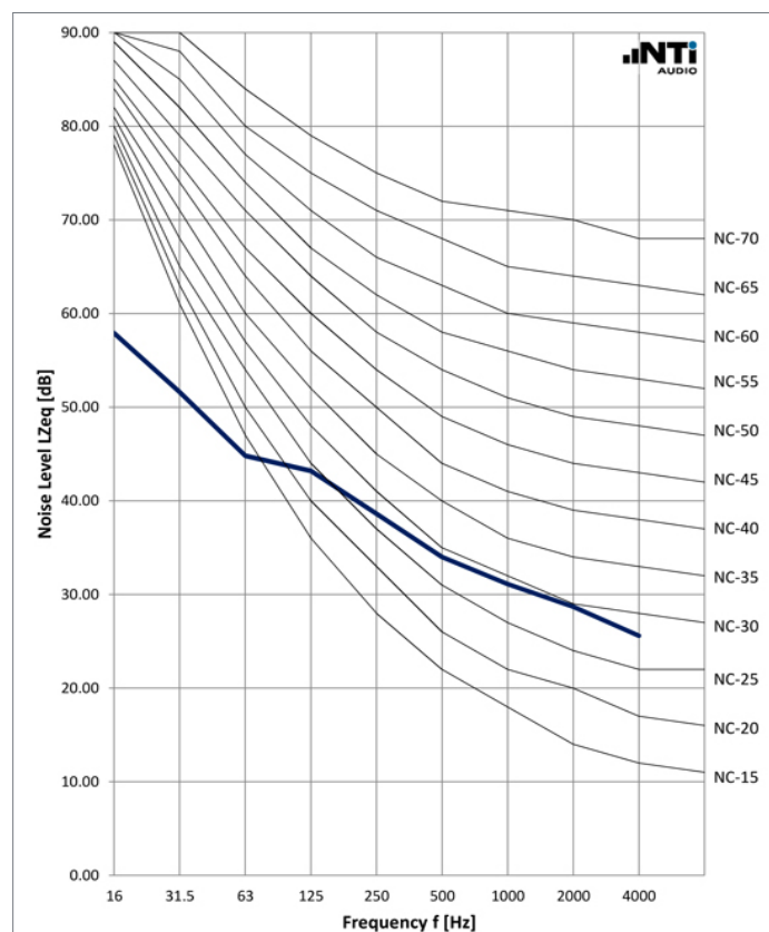
NC Noise Curves
