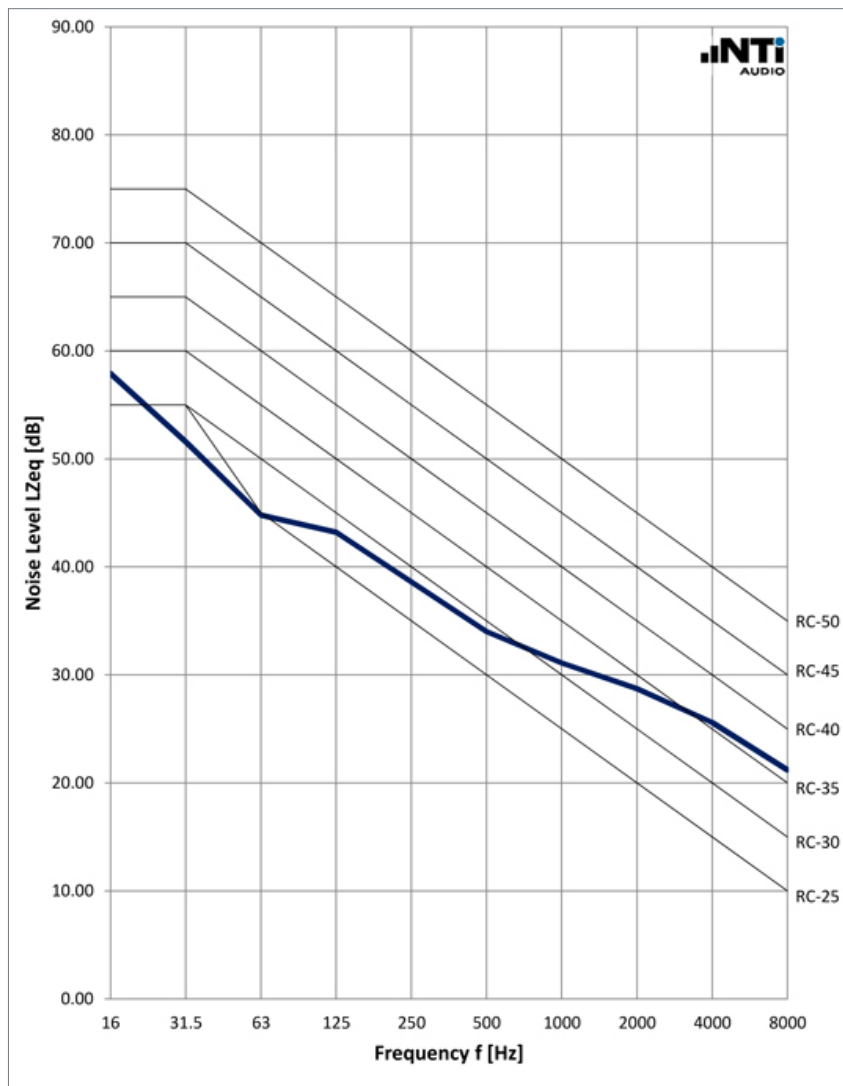
RC Noise Curves
