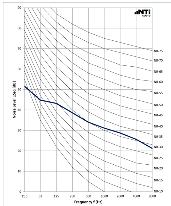
NR Noise Rating Curves
