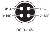
HIROSE 4-pin
