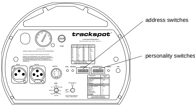
Figure 2-1. Address and personality DIP switches
