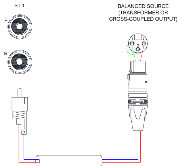
Balanced to Unbalanced input wiring example.
