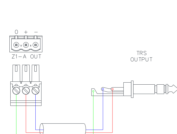
Balanced line output (TRS) wiring example.
