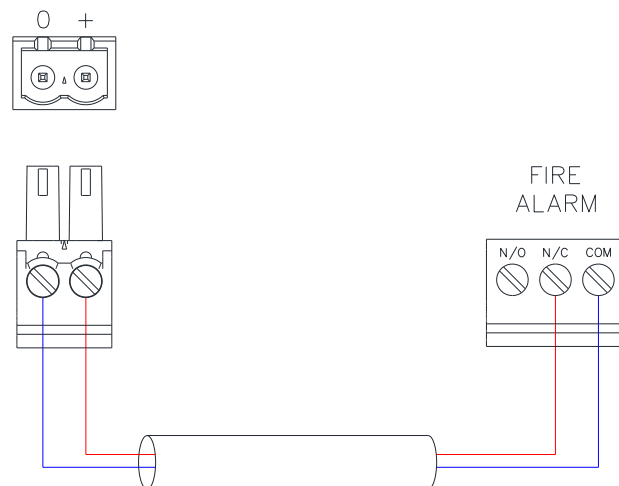
2-wire contact example.
